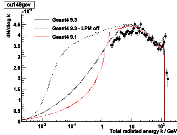
Fig. 1 Bremsstrahlung spectrum for 149 GeV electron beam on a Copper target (4% X_0 ): points – CERN data, 29) histograms – Geant4 simulation results, 9.3 is in agreement with the data.
